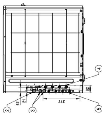
Side View (Piping Connection Ports)
